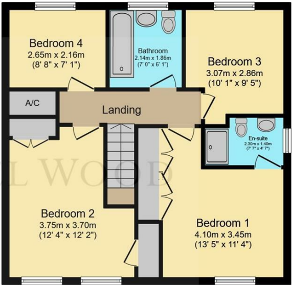
First Floor Floor area 62.5 m 2 (672 sq.ft.)
